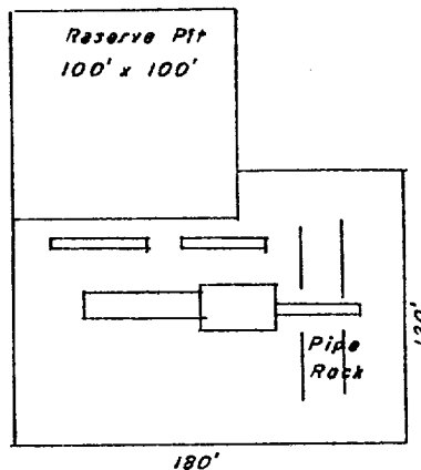
PAD DETAIL
