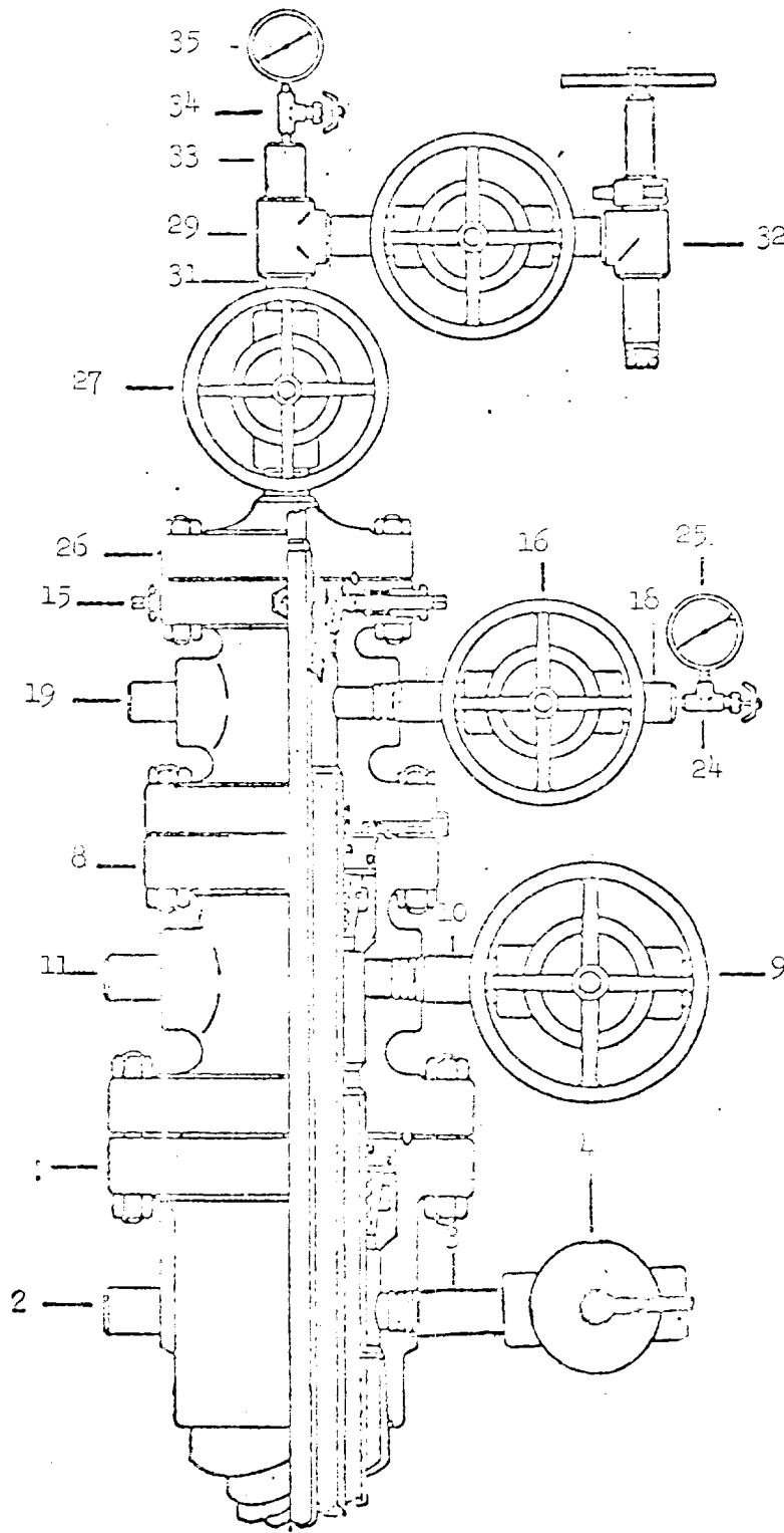
PROPOSED WELLHEAD PLAN FOR THE FEDERAL "G" AND "J" #1
