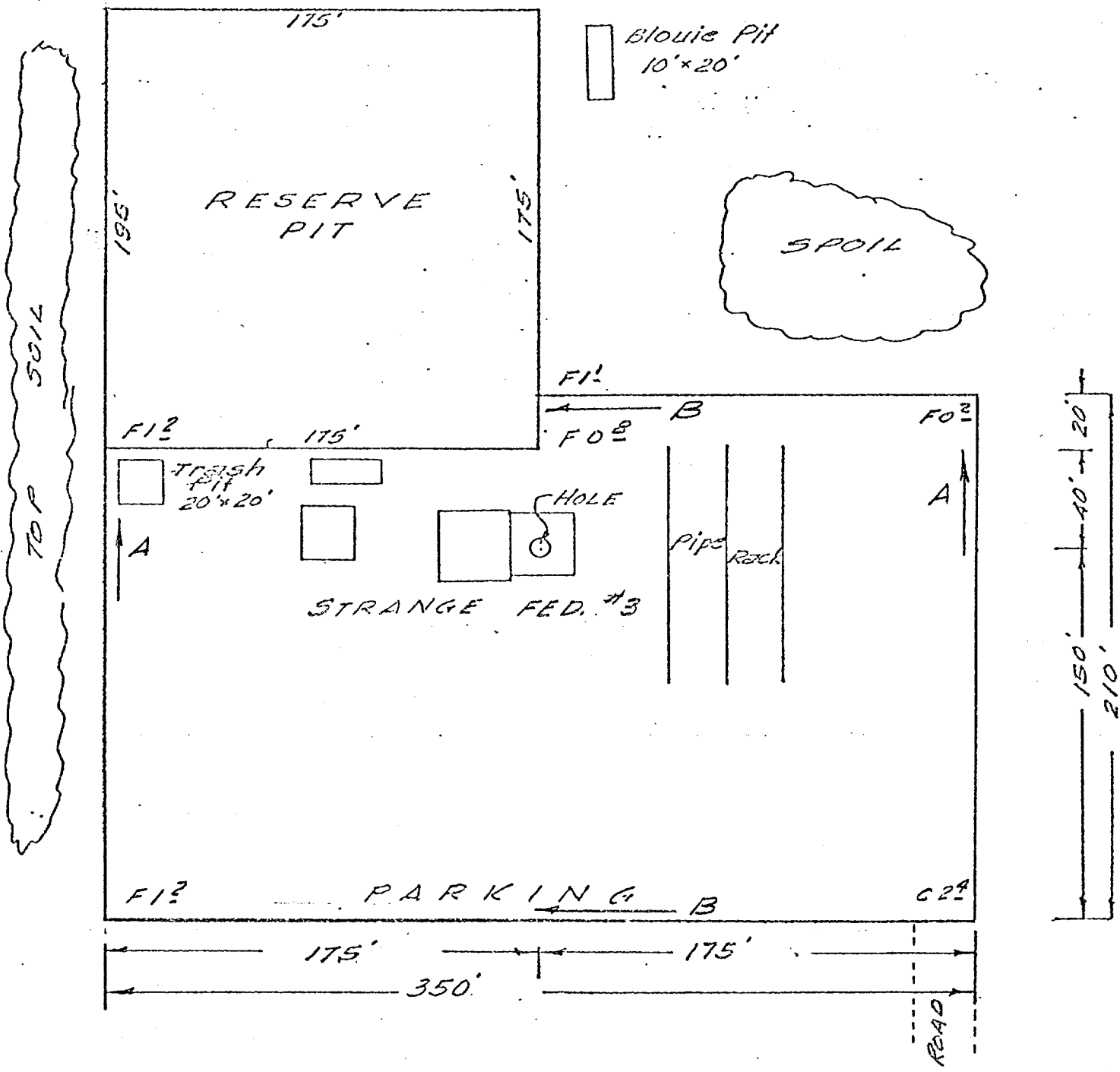
RIG LAYOUT 1" = 60'
