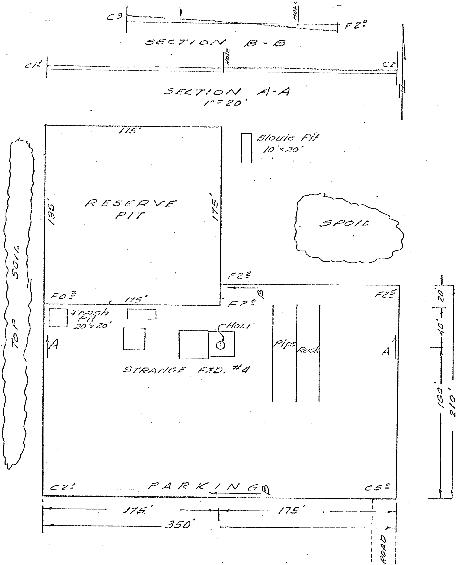
RIG LAYOUT 1" = 60'
