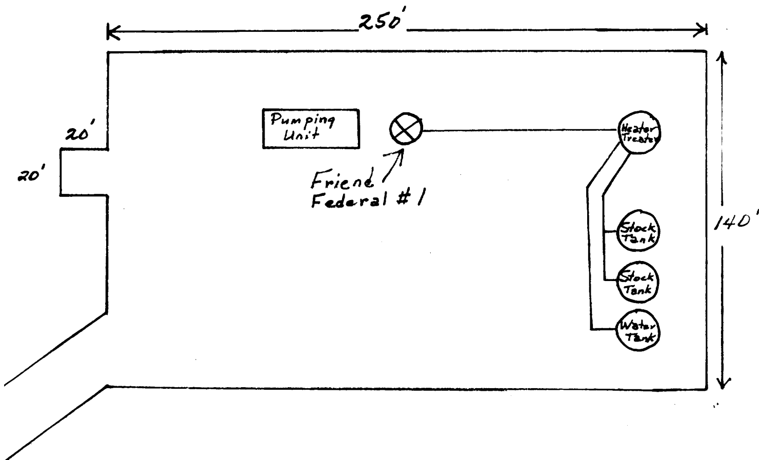
FRIEND FEDERAL #1 PRODUCTION FACILITIES LAYOUT
