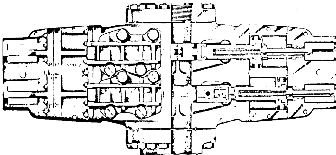
Fig. 52 Shaffer Type E Hydraulic Double Blowout Preventer—Front View
