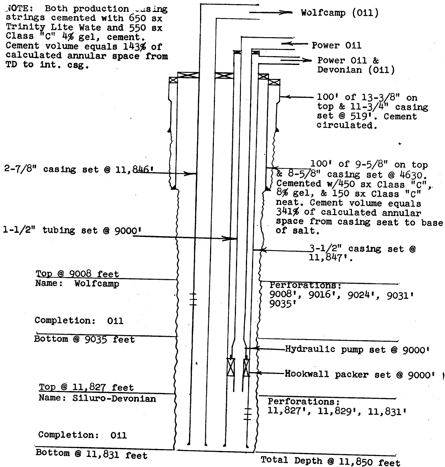
Diagrammatic Sketch
