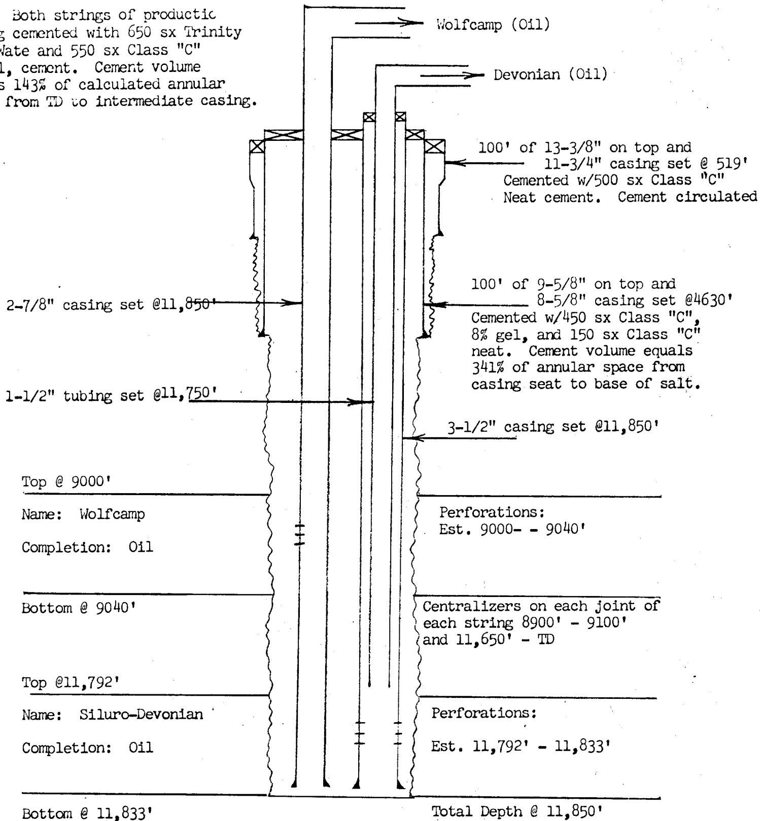
DIAGRAMMATIC SKETCH TEXACO Inc. H. H. Harris Well No. 2 Bronco (Wolfcamp & Siluro-Devonian) Pools Lea County, New Mexico
