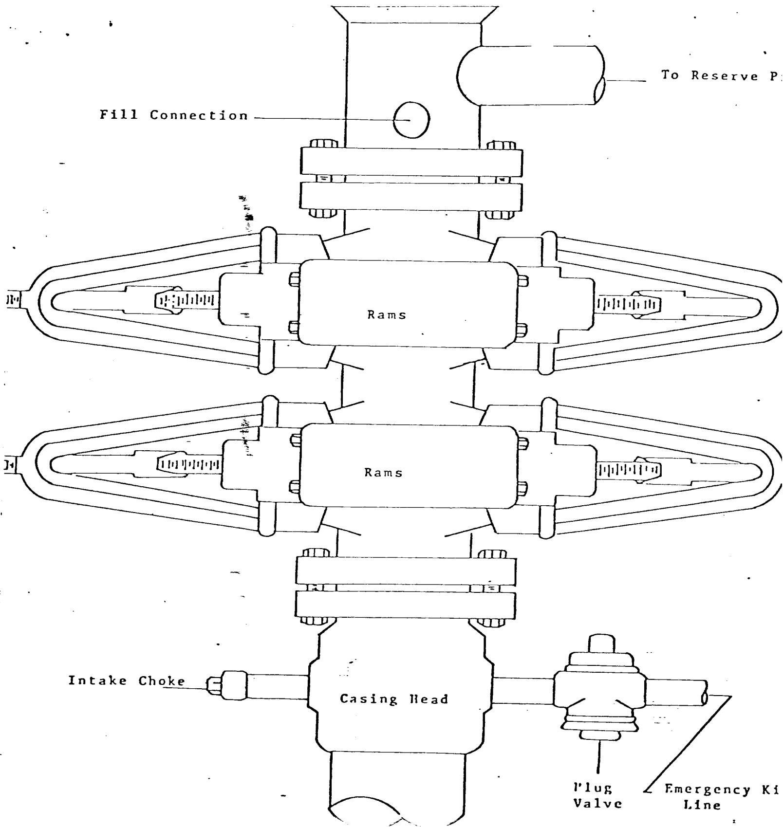
3000 PSI Working Pressure Blowout Preventer Stack
