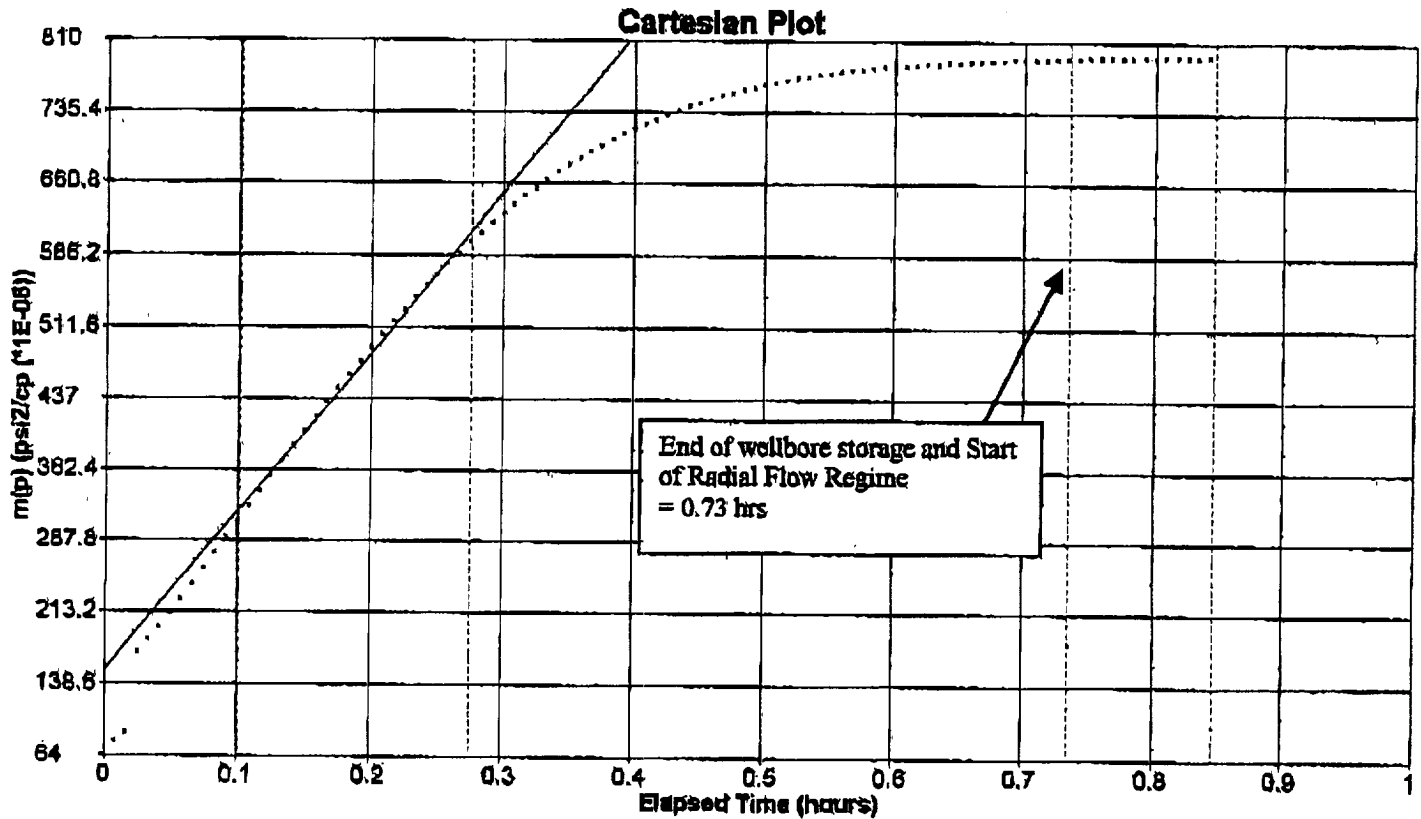
Cartesian Plot - Initial Buildup Data
