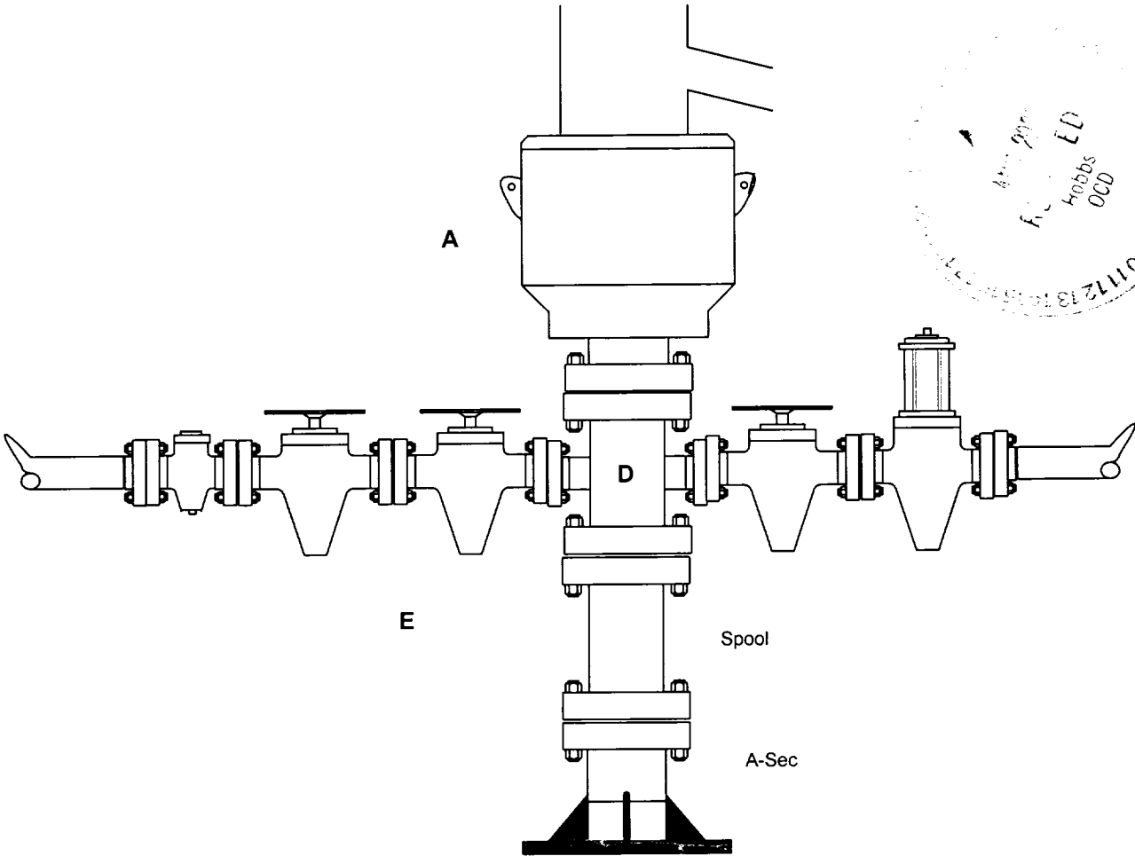
Choke Line
