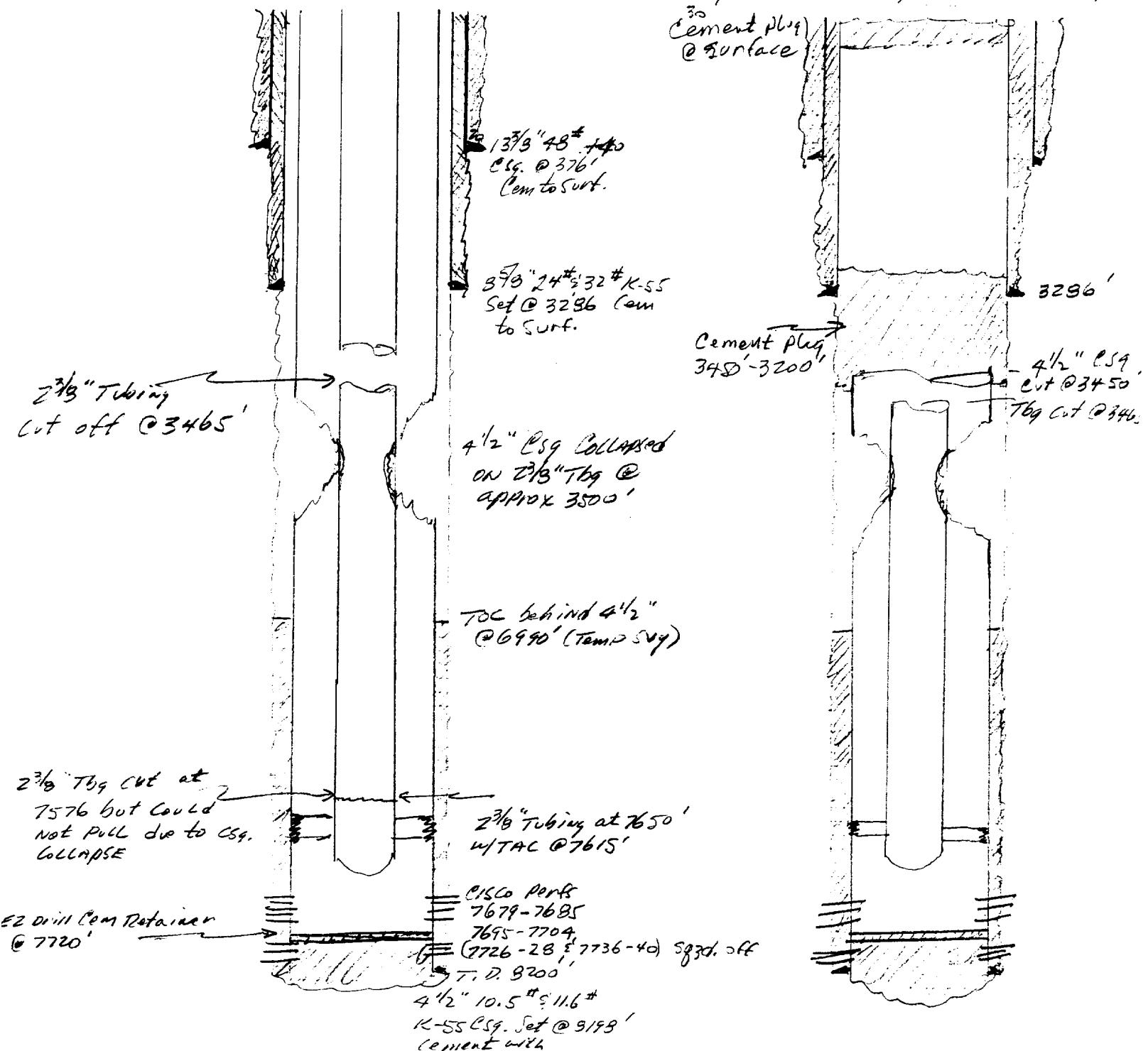
Present Well Bore Configuration
