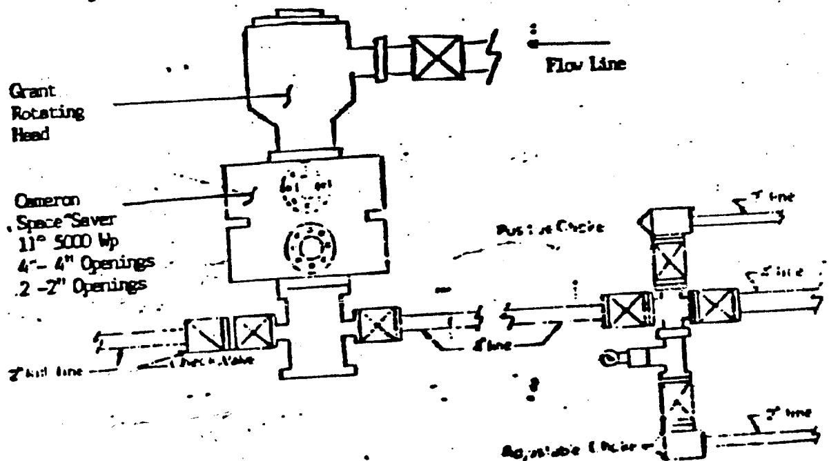
RIG #2 BLOW_OUT EQUIPMENT
