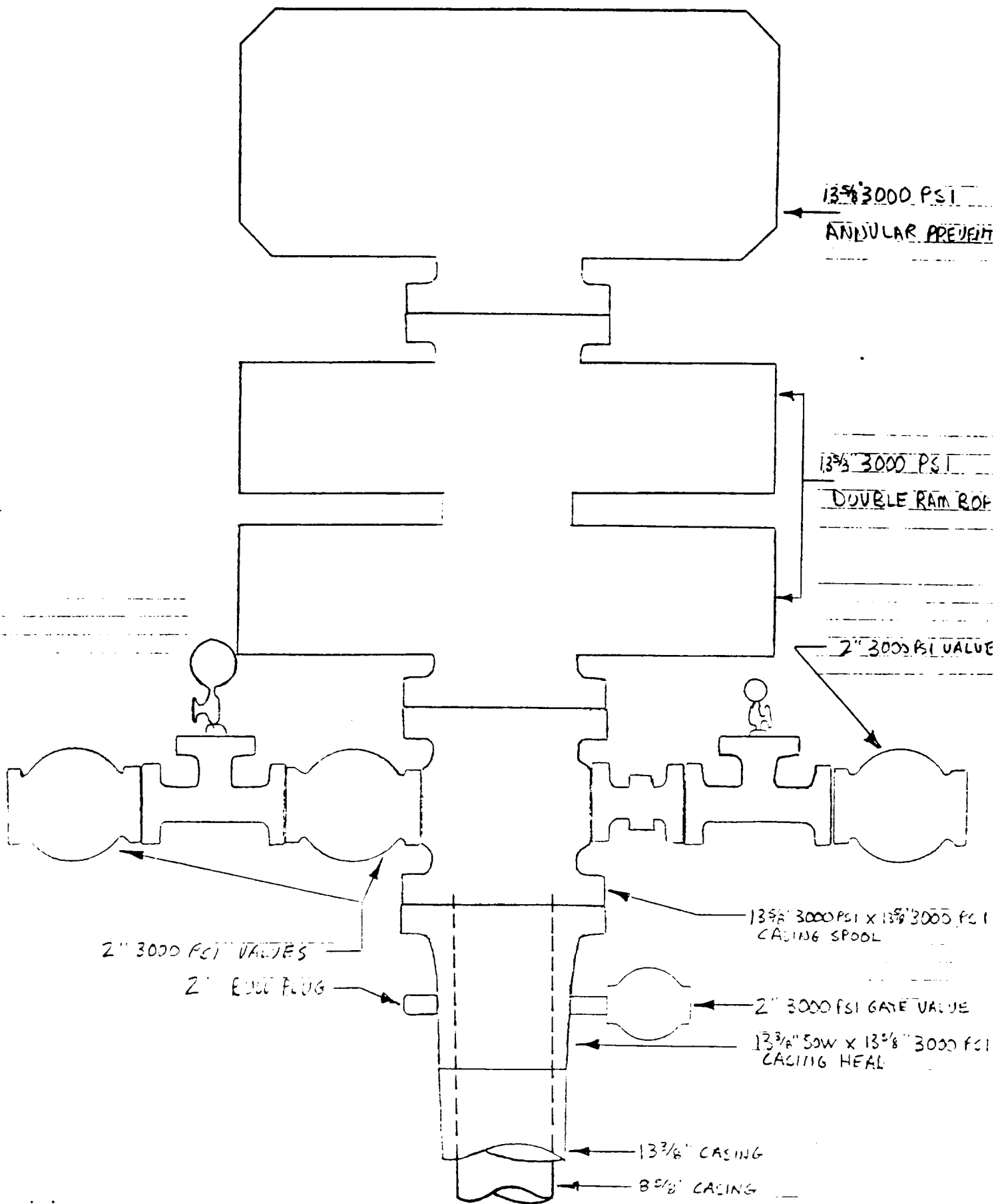
BOP Diagram ANDRUS #1 Lea County New Mexico
