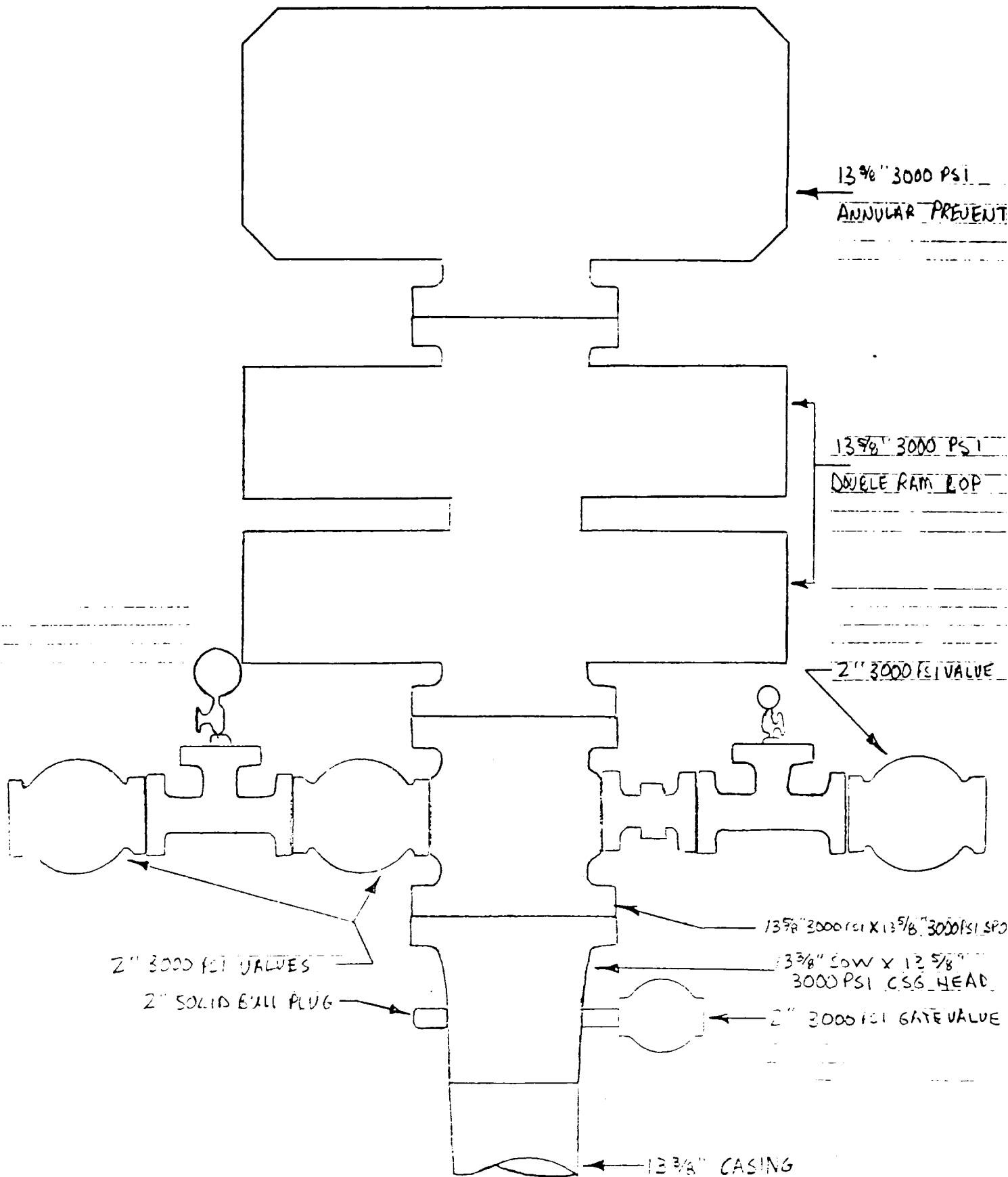
BOP Diagram ANDRUS #1 Lea County New Mexico
