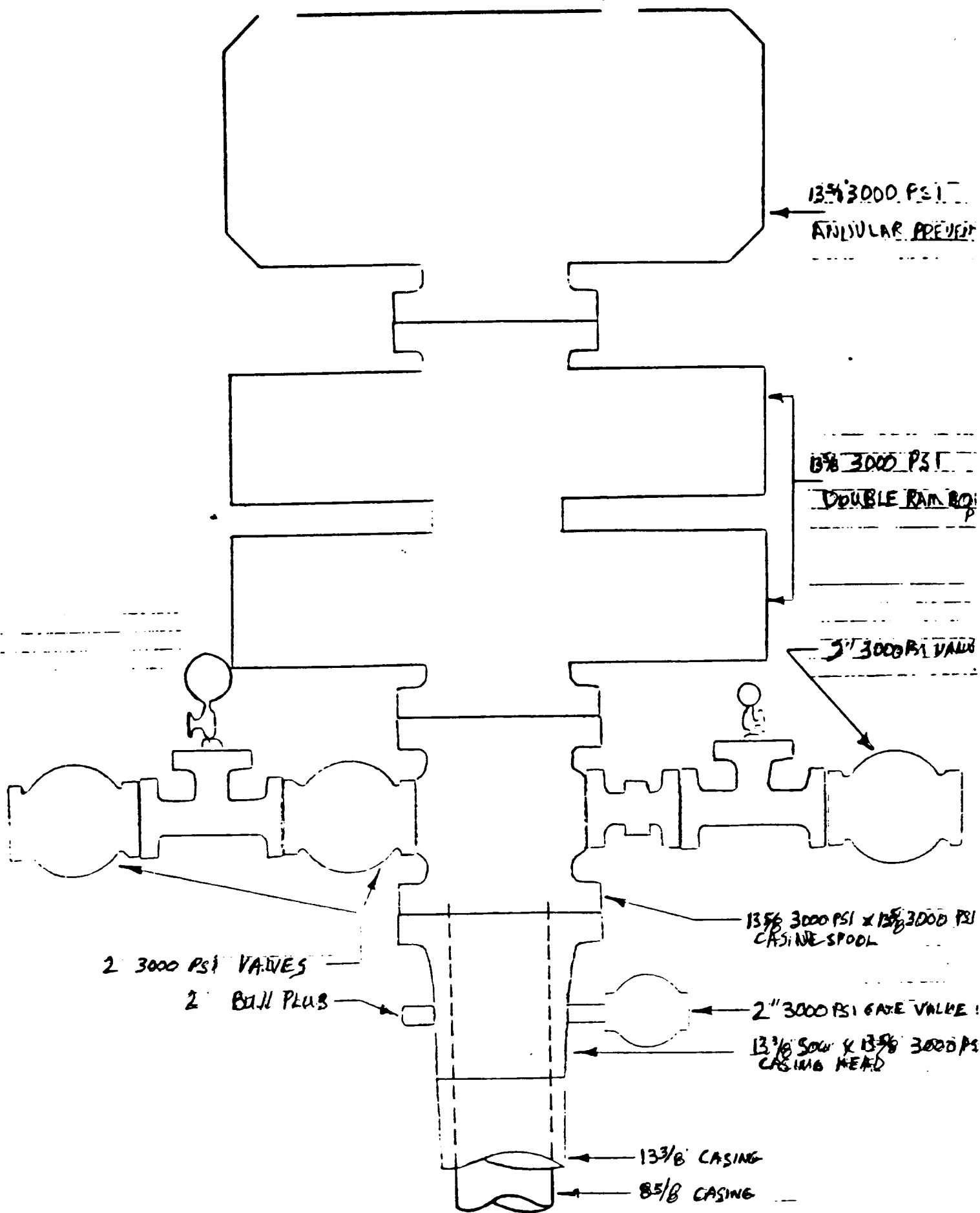
BOP DIAGRAM STATE 4 #1 LEA COUNTY, NEW MEXICO
