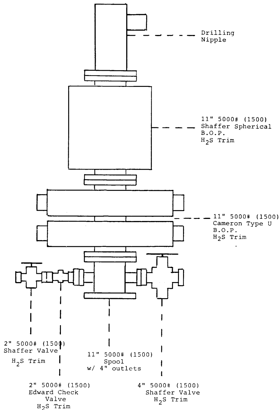
BOP DIAGRAM
