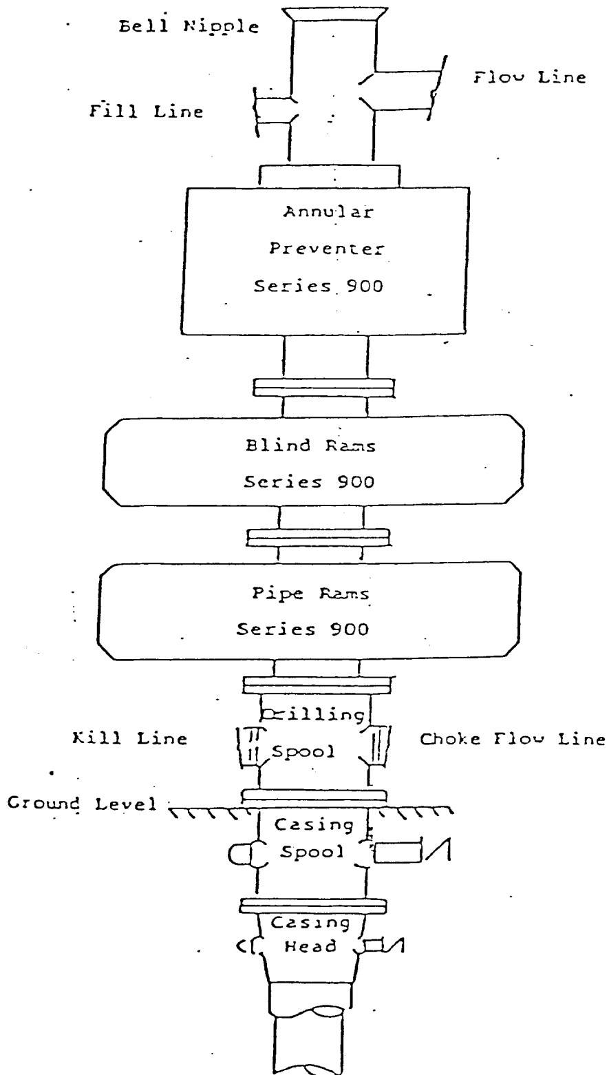
BLOWOUT PREVENTER STACK 3000# WP
