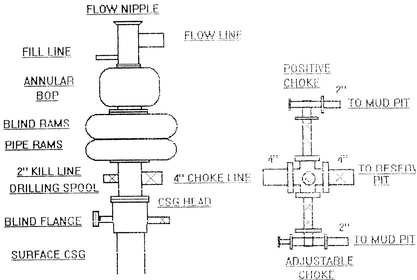
BOP AND CHOKE DIAGRAM GECKO, INC.
