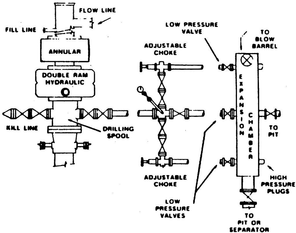
Standard Blowout Preventer Stack
