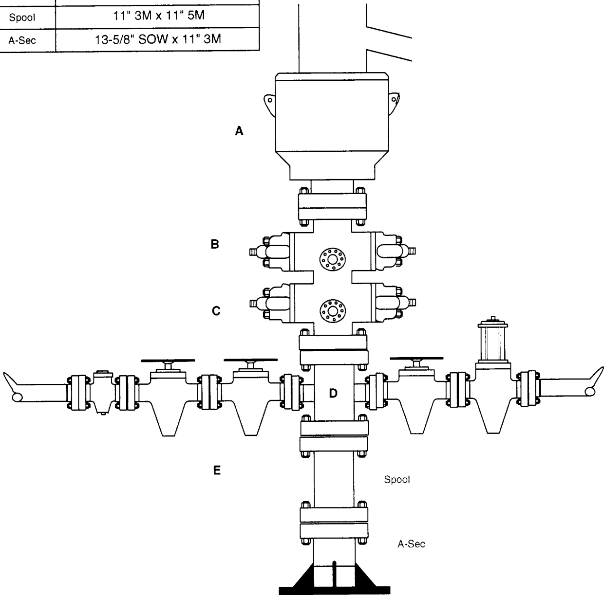
Choke Line
