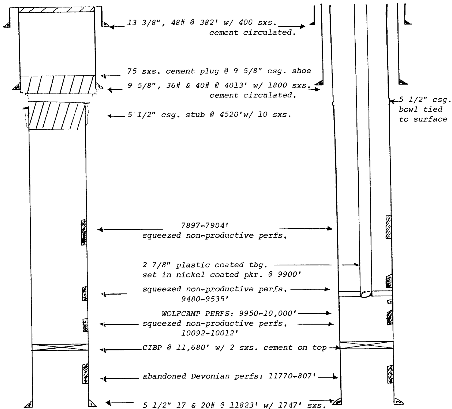
current well bore sketch
