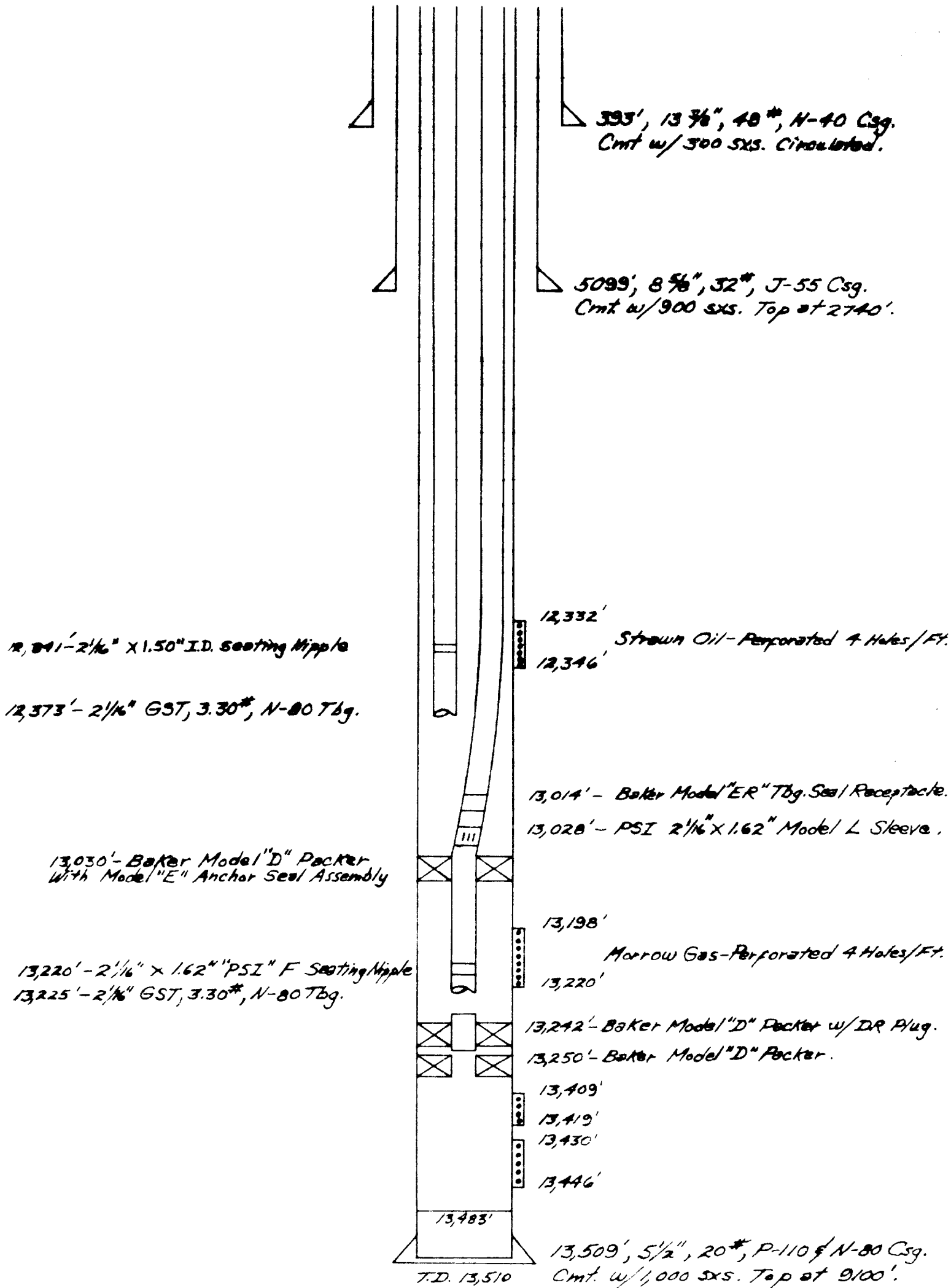
Schematic of Actual Downhole Equipment
