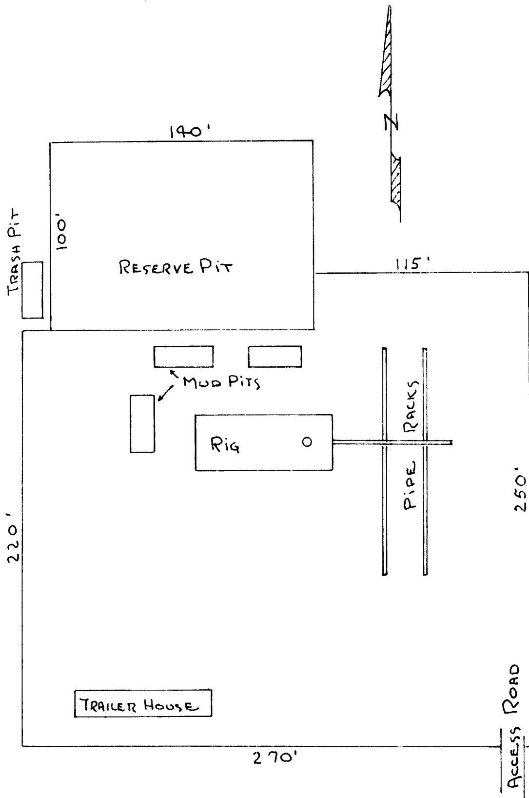
EXHIBIT "C" RIG LAYOUT GENERAL EXPLORATION COMPANY WELL NO. 1 PENNZOIL FEDERAL SCALE: 1" = 50'
