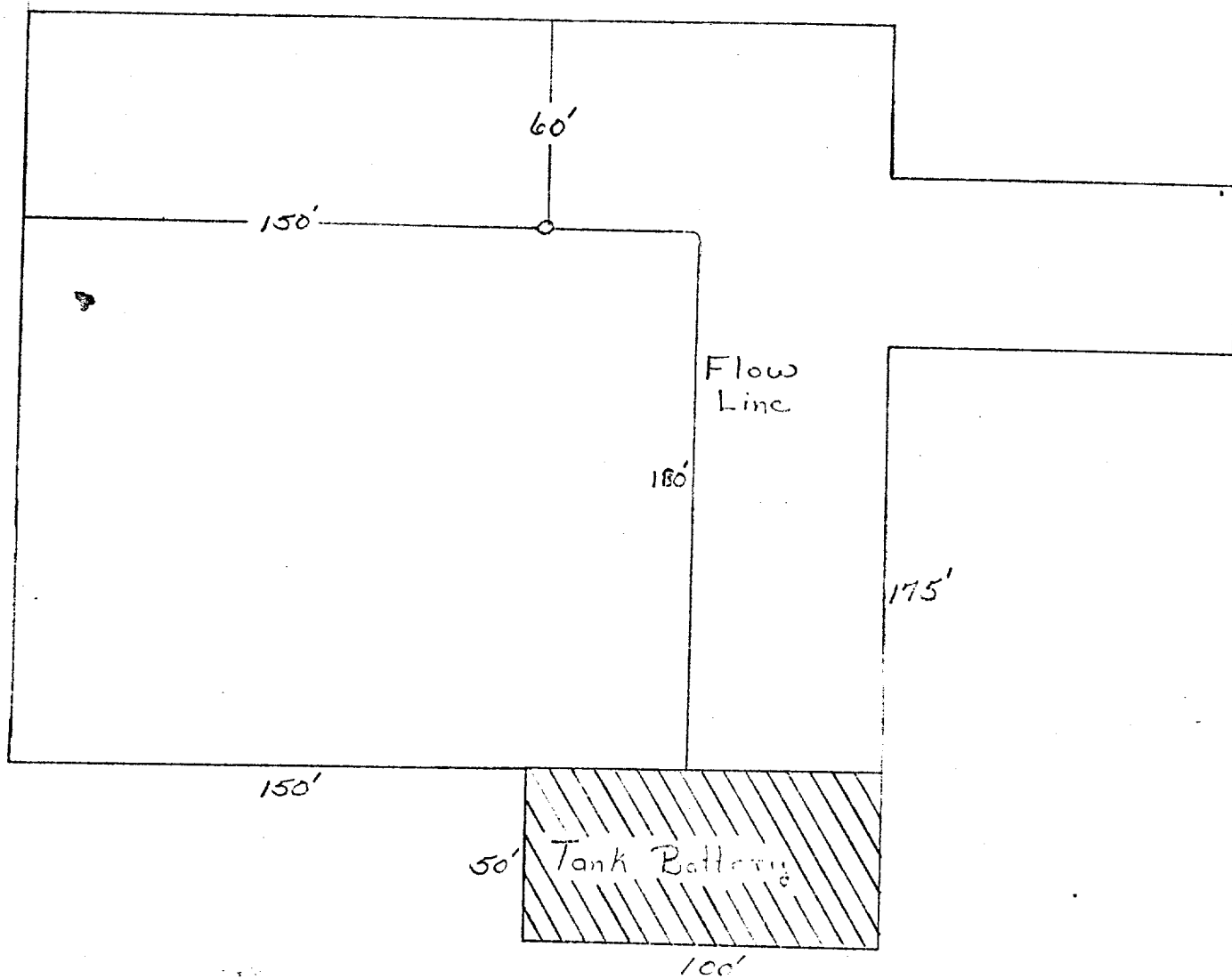
Exhibit "C" Federal Com "4" #1 Sec 4, T19S, R32E Lea Co., New Mexico Drilling Pad Layout
