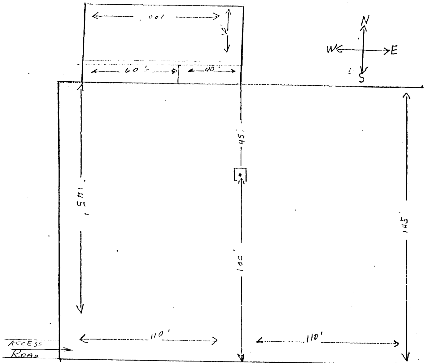
EXHIBIT "D" SEELY OIL CO. McElvain Federal "A", Well No. 1 Pad & Pit Layout
