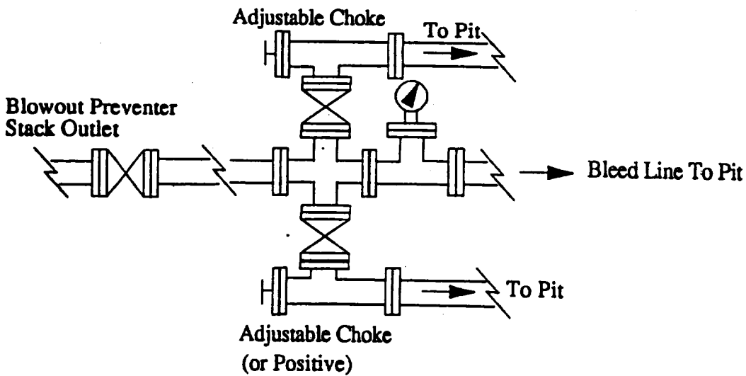
Choke Manifold
