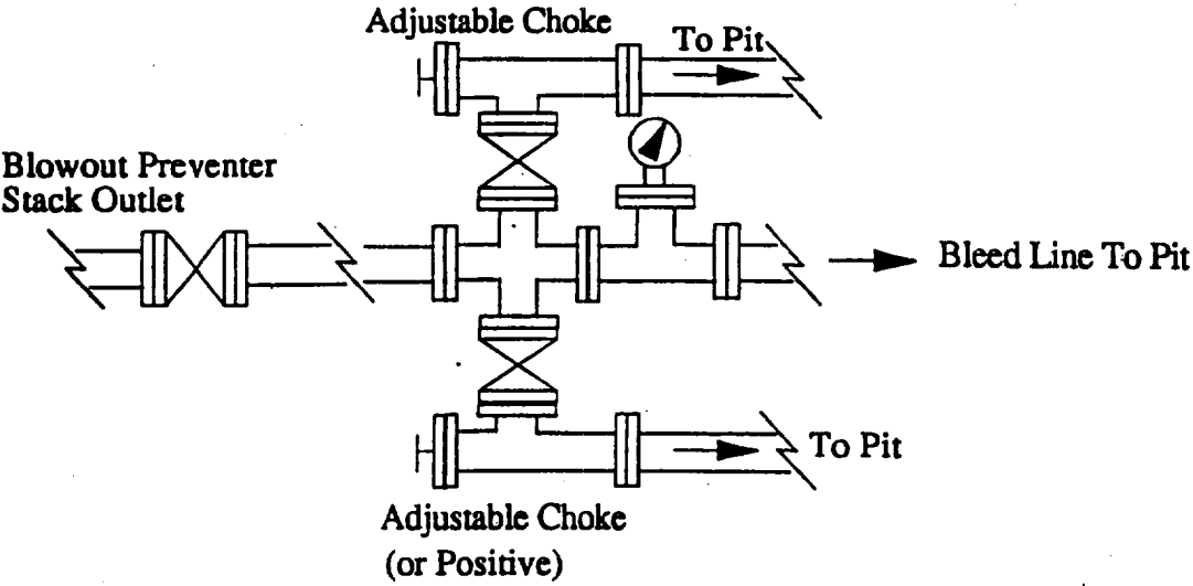
Choke Manifold
