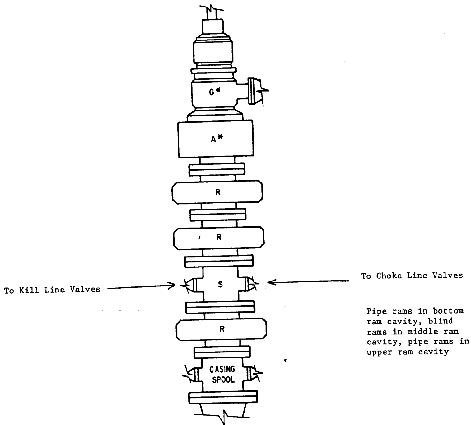
ARRANGEMENT RSRRA*G* Double Ram Type Preventers. Rd. Optional.
