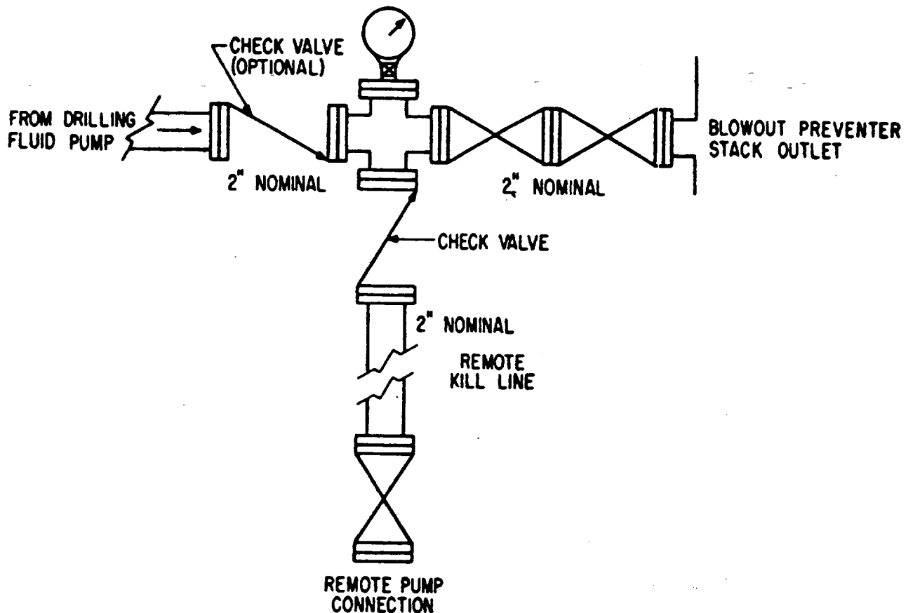
TYPICAL KILL LINE ASSEMBLY FOR 5M, 10M, and 15M RATED WORKING PRESSURE SERVICE — SURFACE IN- STALLATION
