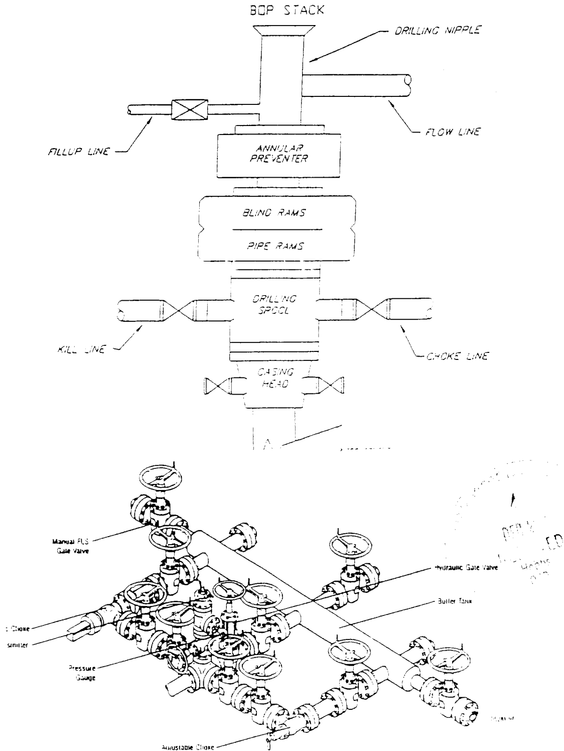
Typical Choke Manifold Designed for Land Drilling Applications
