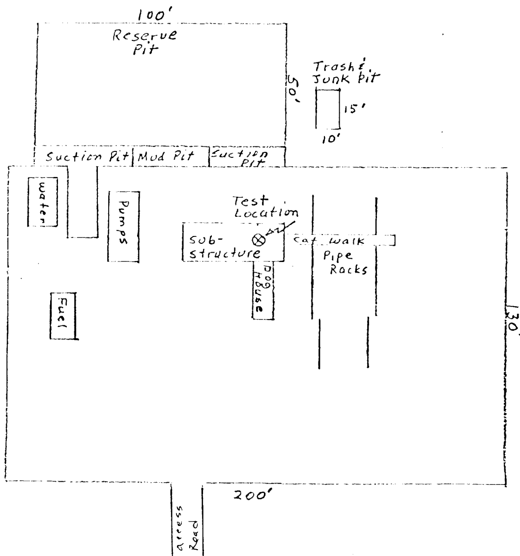
RIG LAY OUT
