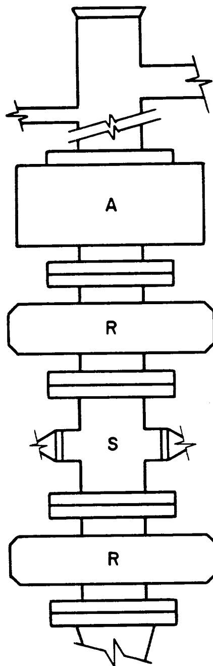
FIG. 2.C.6 ARRANGEMENT RSRA
