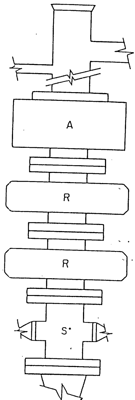
FIG. 2.C.5 ARRANGEMENT S*RA Double Ram Type Preventers. R d , Option:
