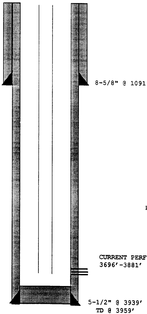
PRESENT WELLBORE
