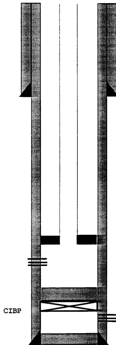
PROPOSED WELLBORE
