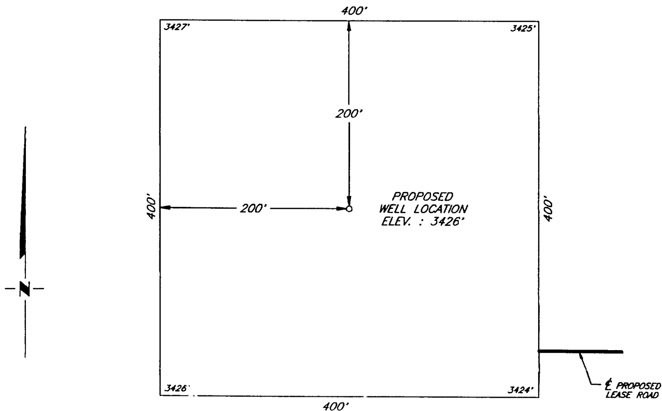
PLAN VIEW 1" = 1000'
