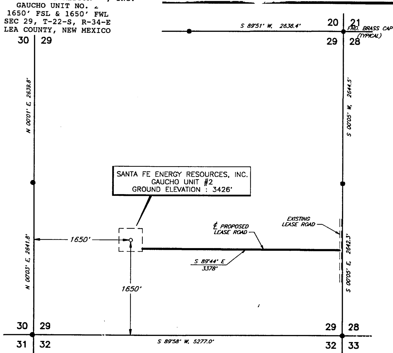
PLAN VIEW 1" = 1000'
