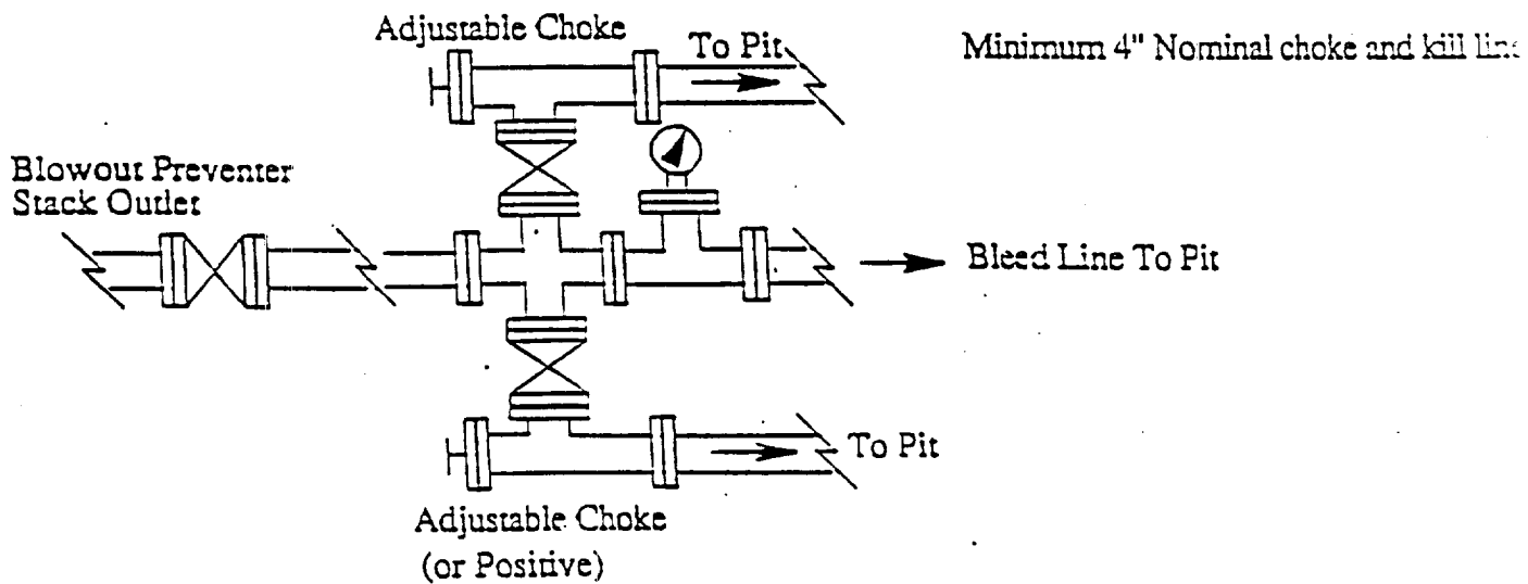
Choke Manifold Requirement (3000 psi WF)
