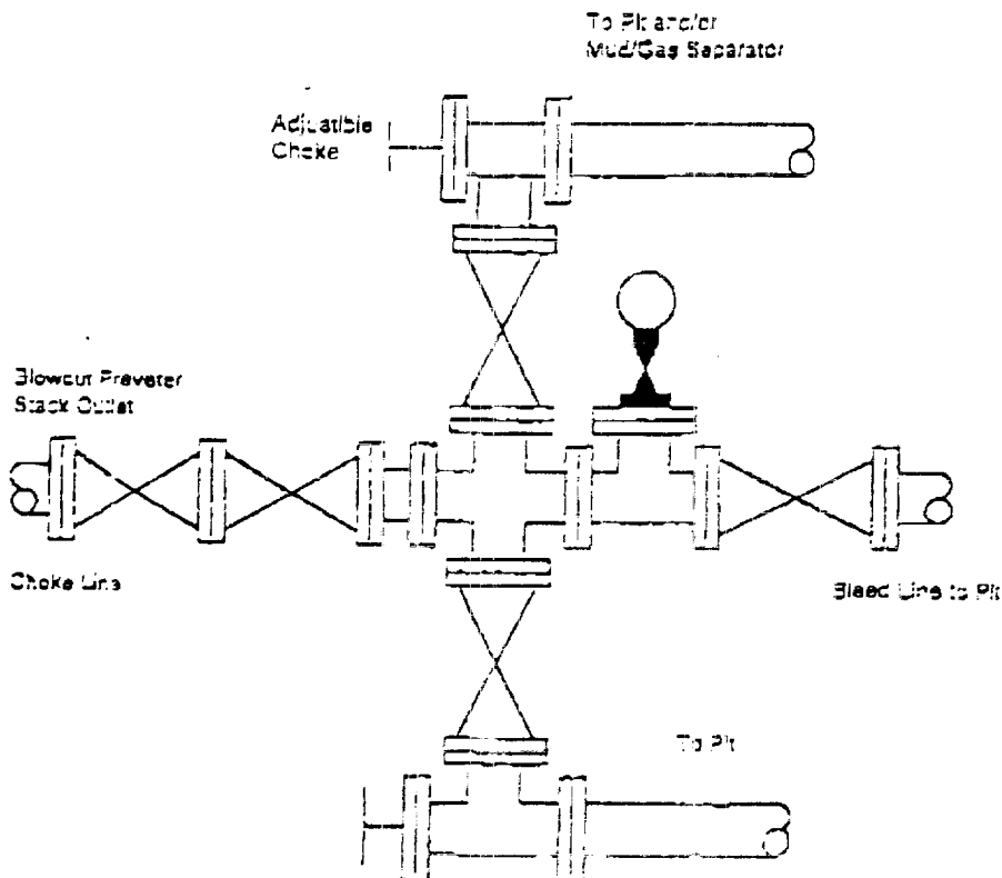
Choke Manifold Assembly for 3M WP System
