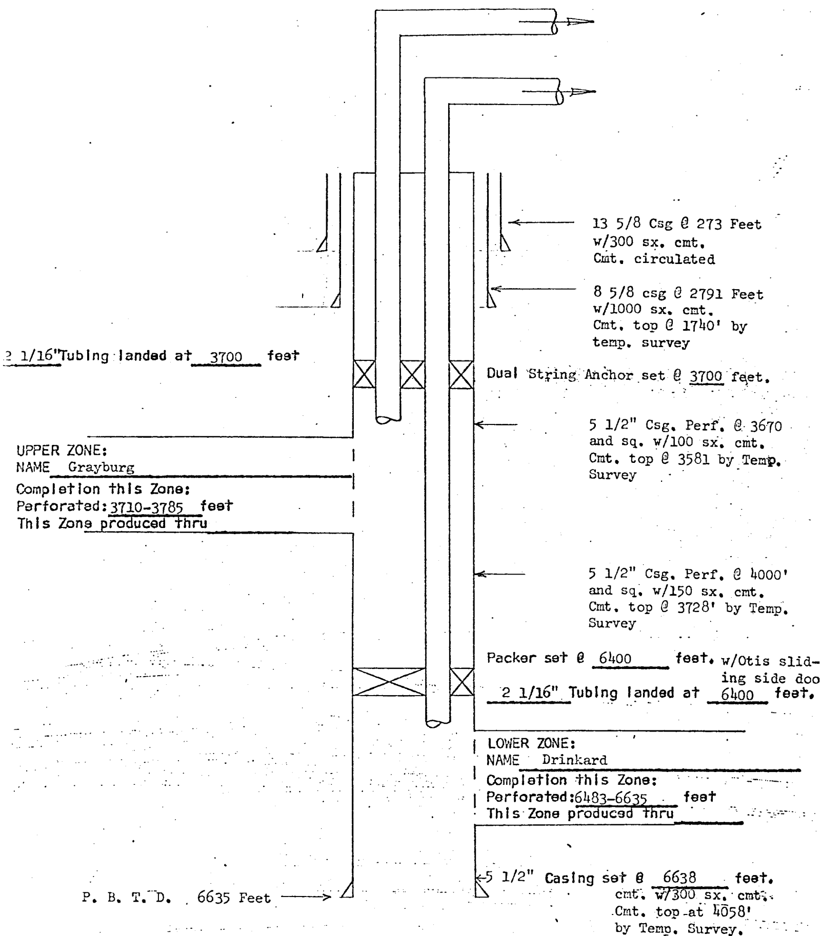
DIAGRAMMATIC SKETCH - DUAL COMPLETION
