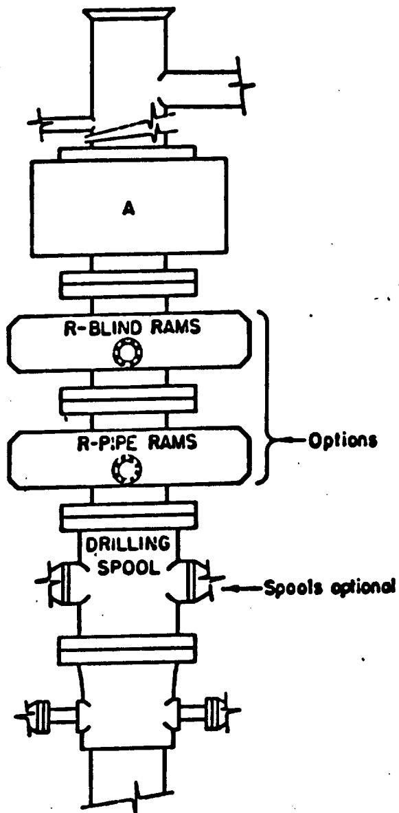
ARRANGEMENT SRRA
