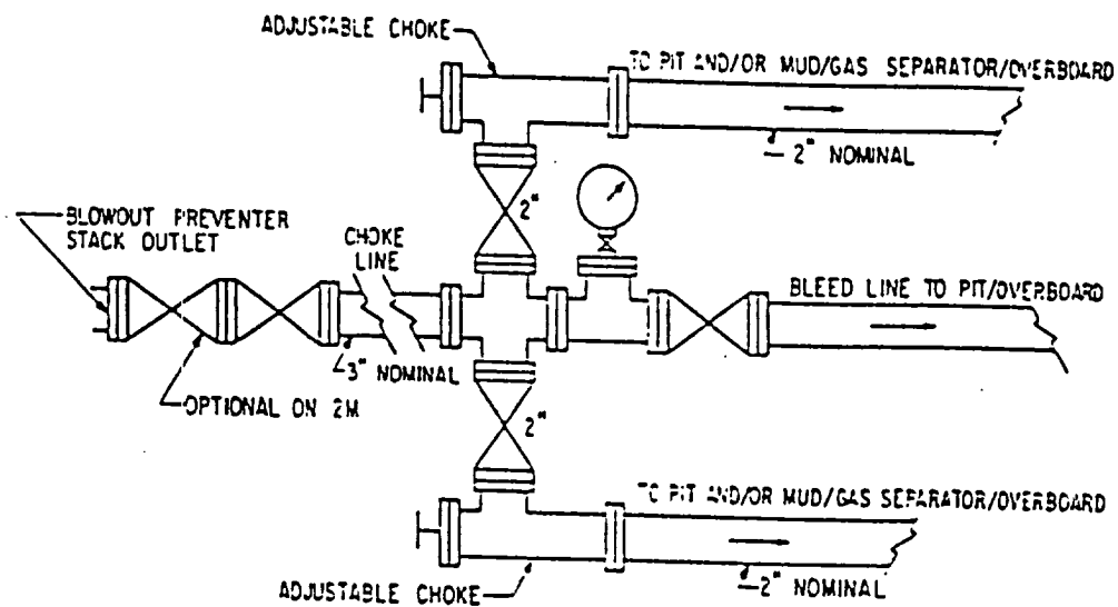
FIG. 3.A.1 EXAMPLE CHOKE MANIFOLD ASSEMBLY FOR 2M AND 3M RATED WORKING PRESSURE SERVICE — SURFACE INSTALLATION
