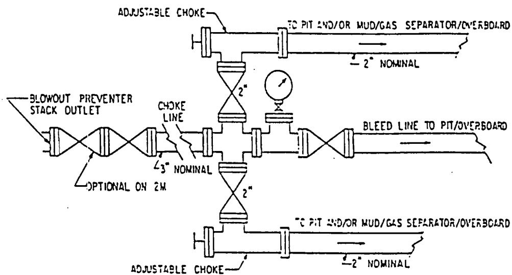
FIG. 3.A.1 EXAMPLE CHOKES MANIFOLD ASSEMBLY FOR 2M AND 3M RATED WORKING PRESSURE SERVICE — SURFACE INSTALLATION
