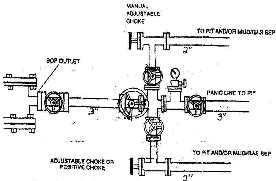
Choke Manifold Schematic
