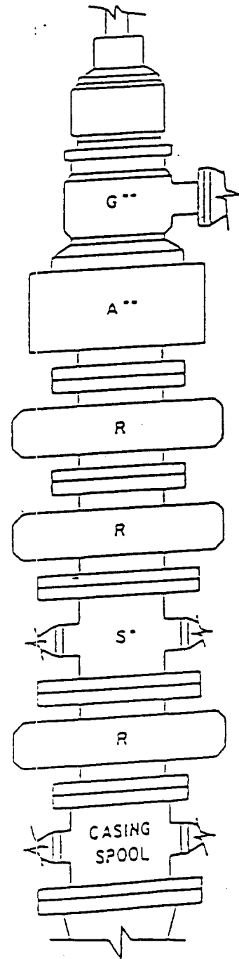
FIG. 2.C.9 ARRANGEMENT RS-PRA-G Double Ram Type Preventers. R 4 Optional
