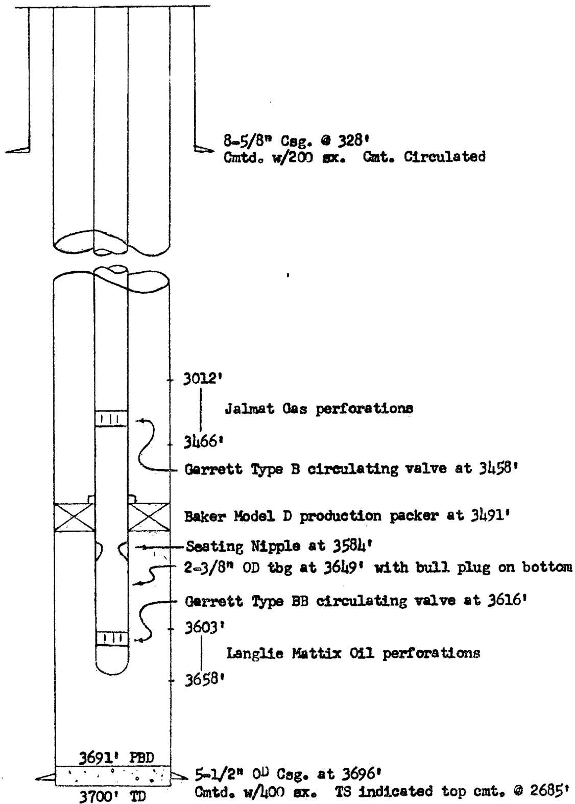
SCHEMATIC DIAGRAM PROPOSED DUAL COMPLETION GULF OIL CORPORATION - J. F. JANDA (NCT-H) NO. 3 LANGLIE MATTIX OIL - JALMAT GAS Unit J, Sec. 11, T-23-S, R-36-E
