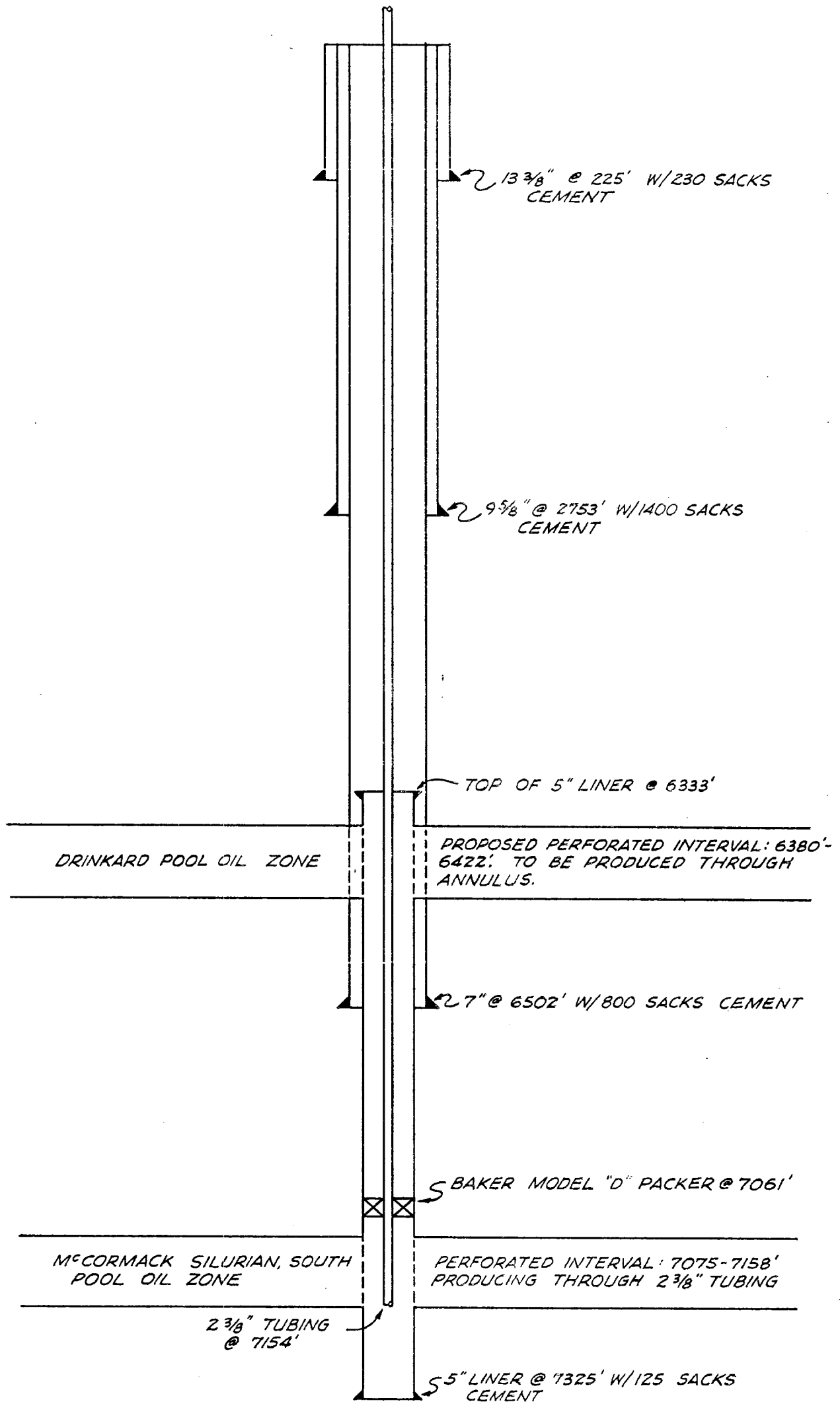
DIAGRAMMATIC SKETCH OF PROPOSED DUAL COMPLETION DRINKARD POOL OIL ZONE & MCCORMACK SILURIAN, SOUTH POOL OIL ZONE
