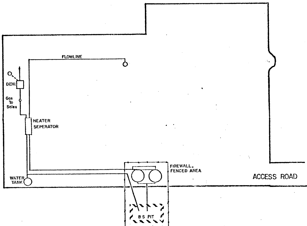
TANK BATTERY LAYOUT
