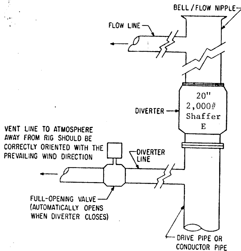
FIG. 2.A.2 TYPICAL DIVERTER SYSTEM — SURFACE INSTALLATION
