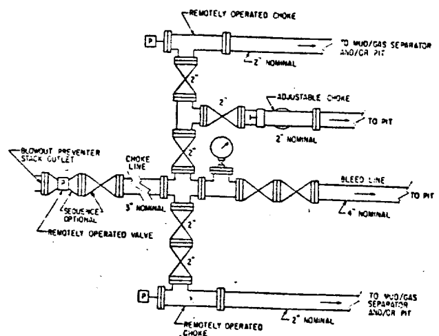
CHOKE MANIFOLD All Valves to be 5,000 psi
