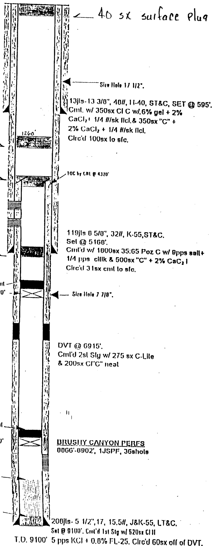
Current Wellbore Diagram
