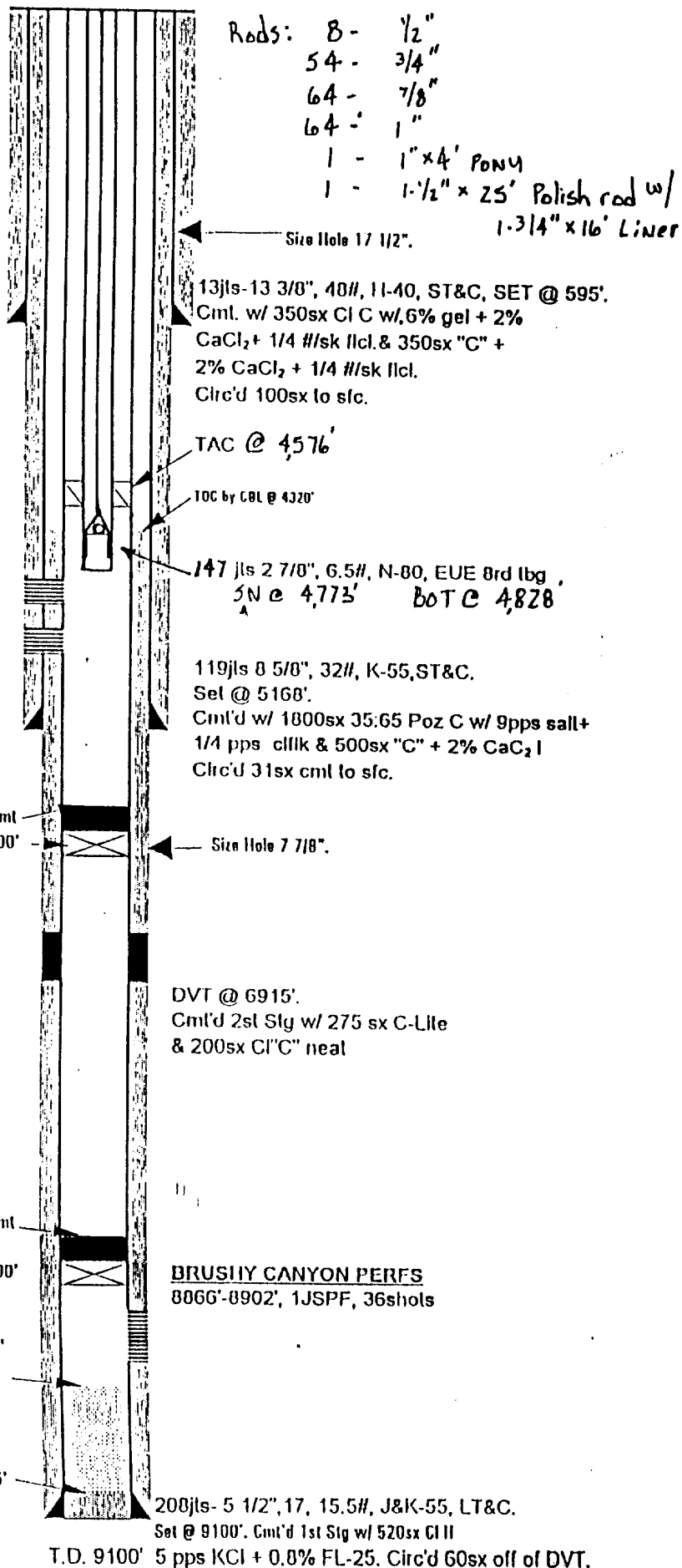
Current Wellbore Diagram
