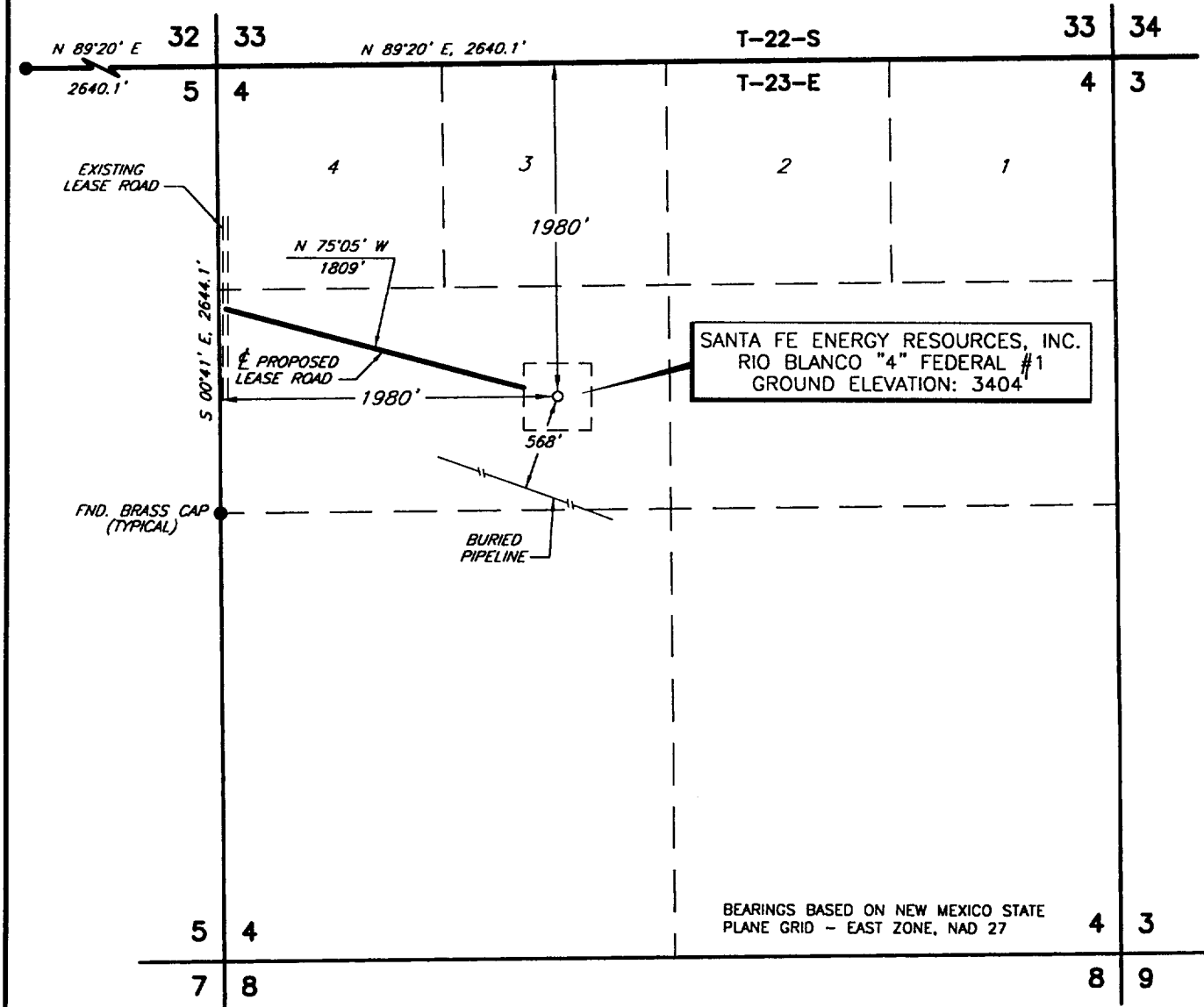
PLAN VIEW 1" = 1000'
