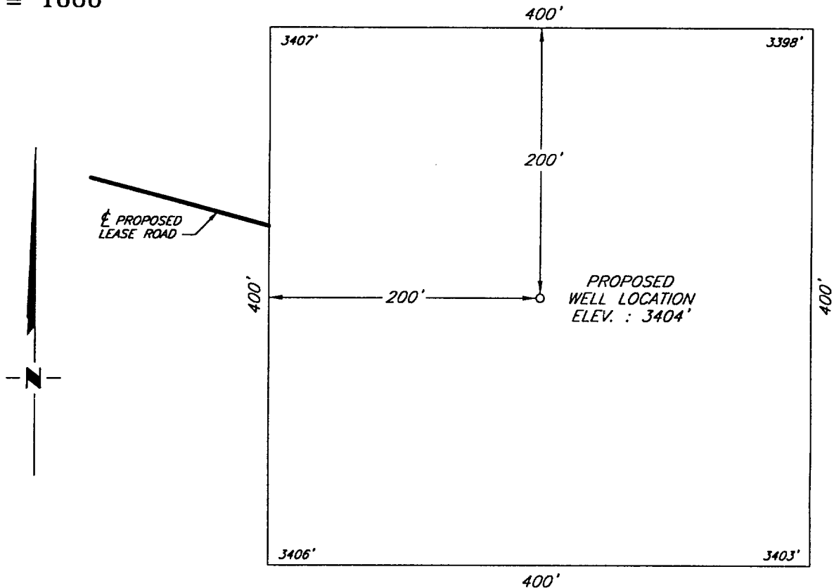
DETAIL VIEW 1" = 100'
